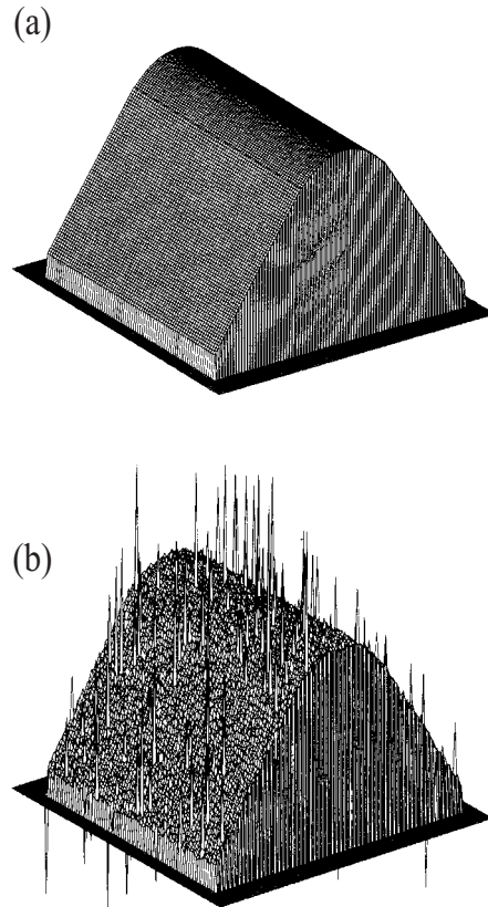
Figure 5: (a) Smooth join surface and (b) surface contaminated with added Gaussian noise and outliers
