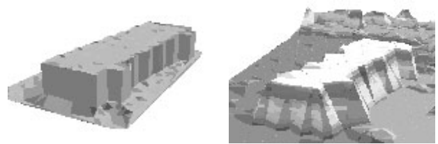
Figure 5: Perspective view of the building model. The left image shows the model created from photogrammetrically measured points. The right image is a TIN model of the laser points. The photogrammetric model is superior because twice as many points were measured. The building outline (breakline) was also measured.
