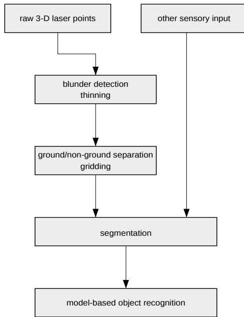
Figure 1: Major processing steps of raw laser data. A popular sequence is to interpolate the irregularly distributed laser points to a grid, followed by object modeling. A conceptually more pleasing sequence includes segmentation (preferably without gridding), before object modeling is attempted.
