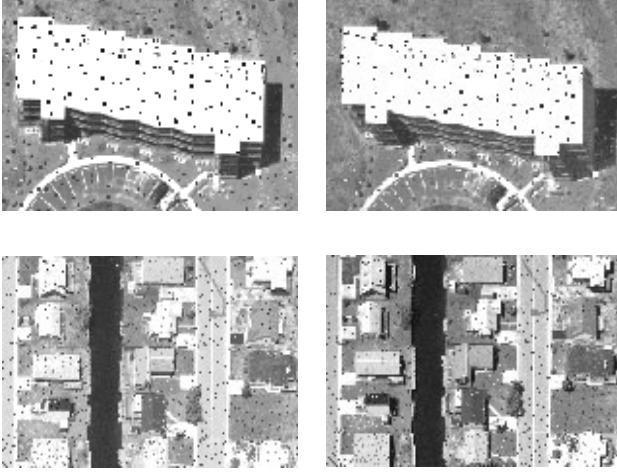
Figure 4: Illustration of projecting the laser points to a stereopair (backprojection). The stereopair can be viewed on an analytical plotter or on a softcopy workstation. If the laser points are not on the visible surface, defined by the stereo image, differences can be measured and analyzed. This technique is also very useful to examine "problematic" laser points, for example around buildings. It is also possible to perform the comparison automatically by image matching techniques (see text for details).
