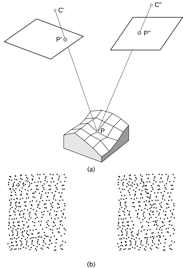
Figure 2: Figure (a) illustrates the principle of generating a stereogram from a raw laser data set. Based on an assumed exterior orientation, synthetic laser images are computed that can be viewed stereoscopically on stereoscopes, analytical plotters, or softcopy workstations. The latter possibility is appealing for it allows to browse through large data sets with the possibility to measure. In (b), a stereogram of laser points is generated. It contains the apartment building shown in Fig. 3. Viewed under a stereoscope, a vivid 3-D impression of the building and its surrounding appears.
