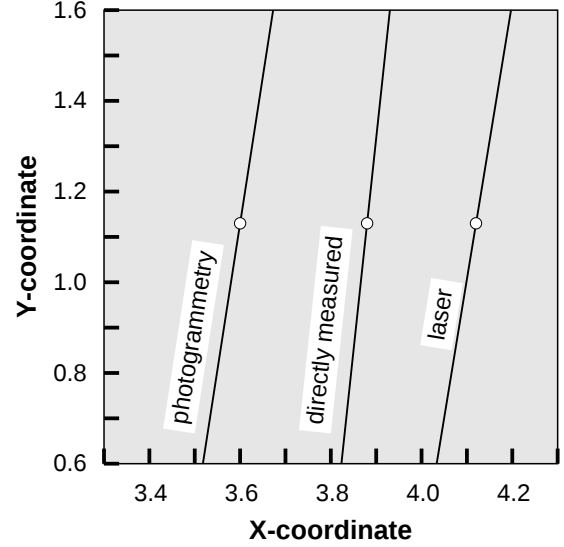
Figure 9: The roof ridge was computed by intersecting the two roof planes, obtained from laser roof points and from DEM measurements. The edge was also directly measured. The figure shows the three roof edges, together with the reference points whose values are listed in Table 2.
